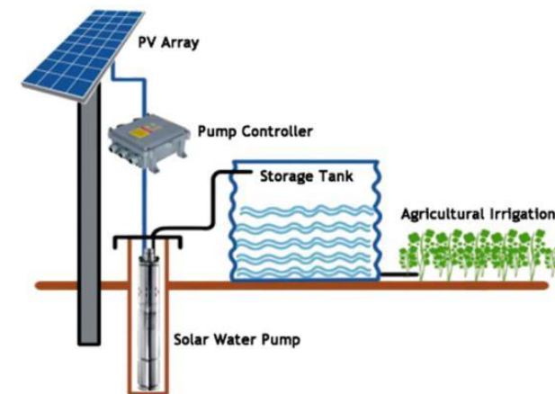
Figure 1. Solar pumping system
